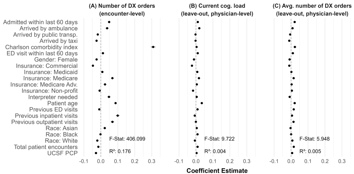
Figure 2: Covariate Balance
