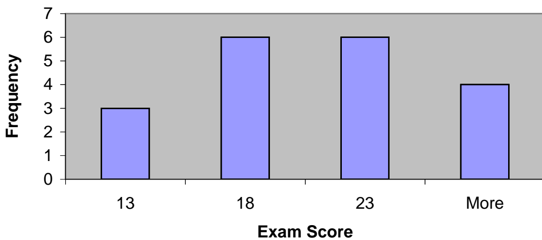
Histogram
